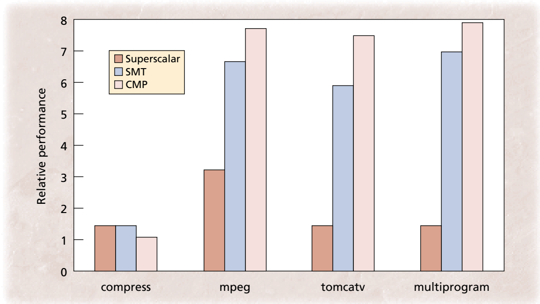
Figure 2. Relative performance of superscalar, simultaneous multithreading, and chip multiprocessor architectures compared to a baseline, 2-issue superscalar architecture.
