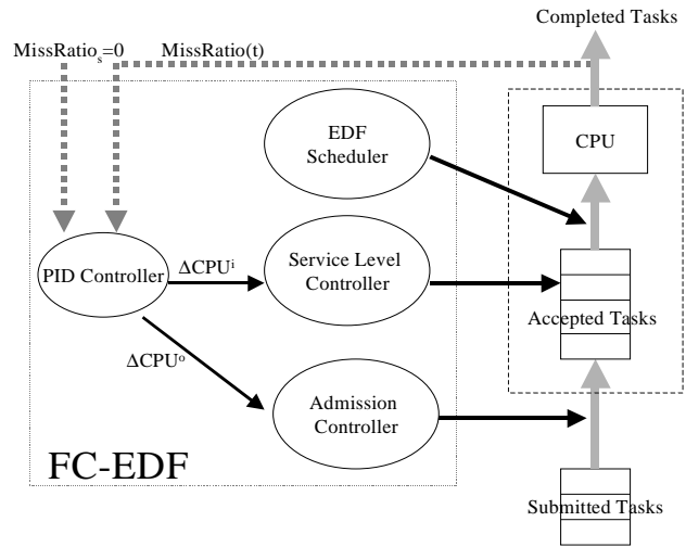
Figure 2 Architecture of FC-EDF
