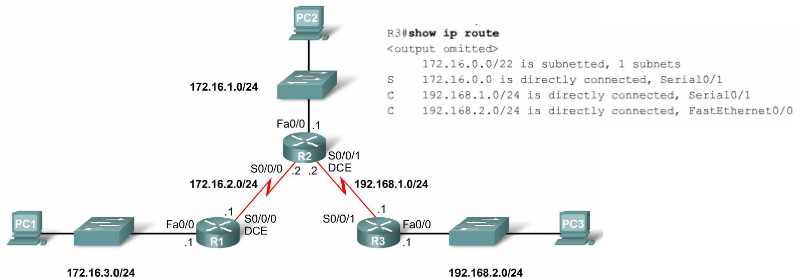
Static routes and packet forwarding
