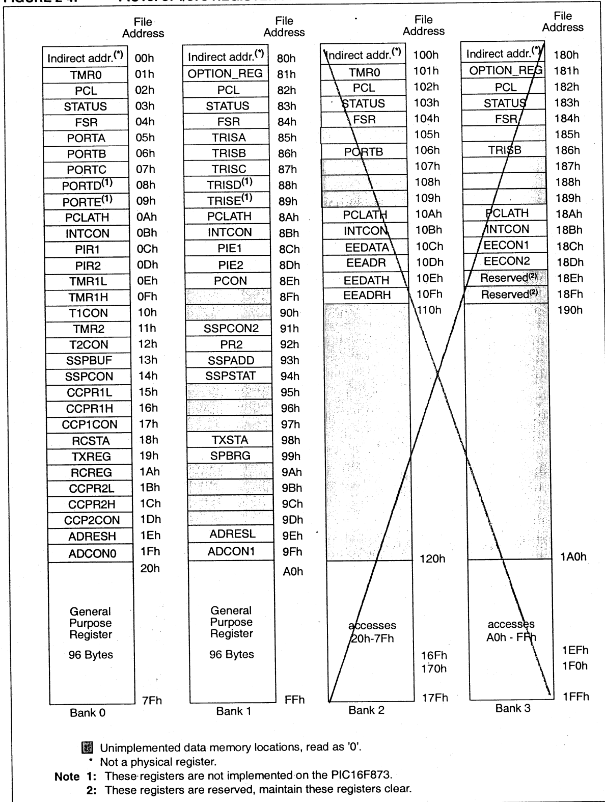
FIGURE 2-4: PIC16F874/873 REGISTER FILE MAP
